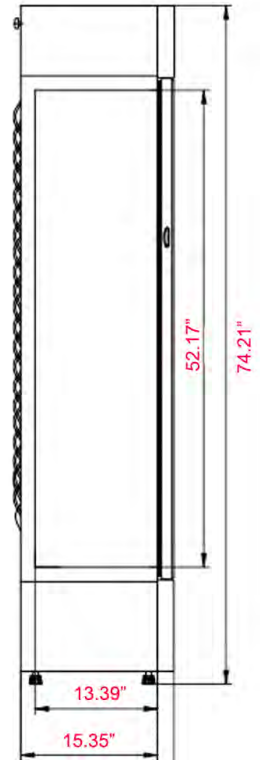
SIDE VIEW
