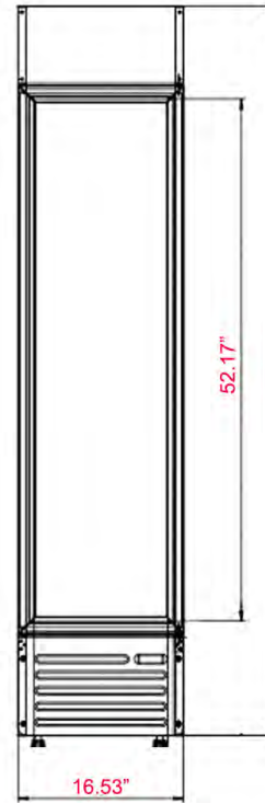
FRONT VIEW
