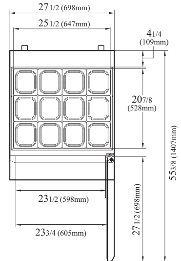
PLAN VIEW
