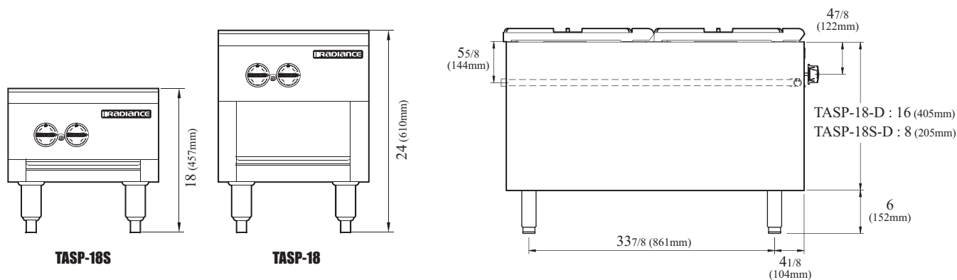
FRONT VIEW
