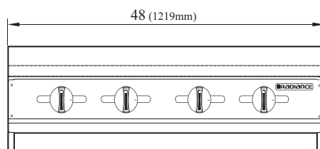
FRONT VIEW
