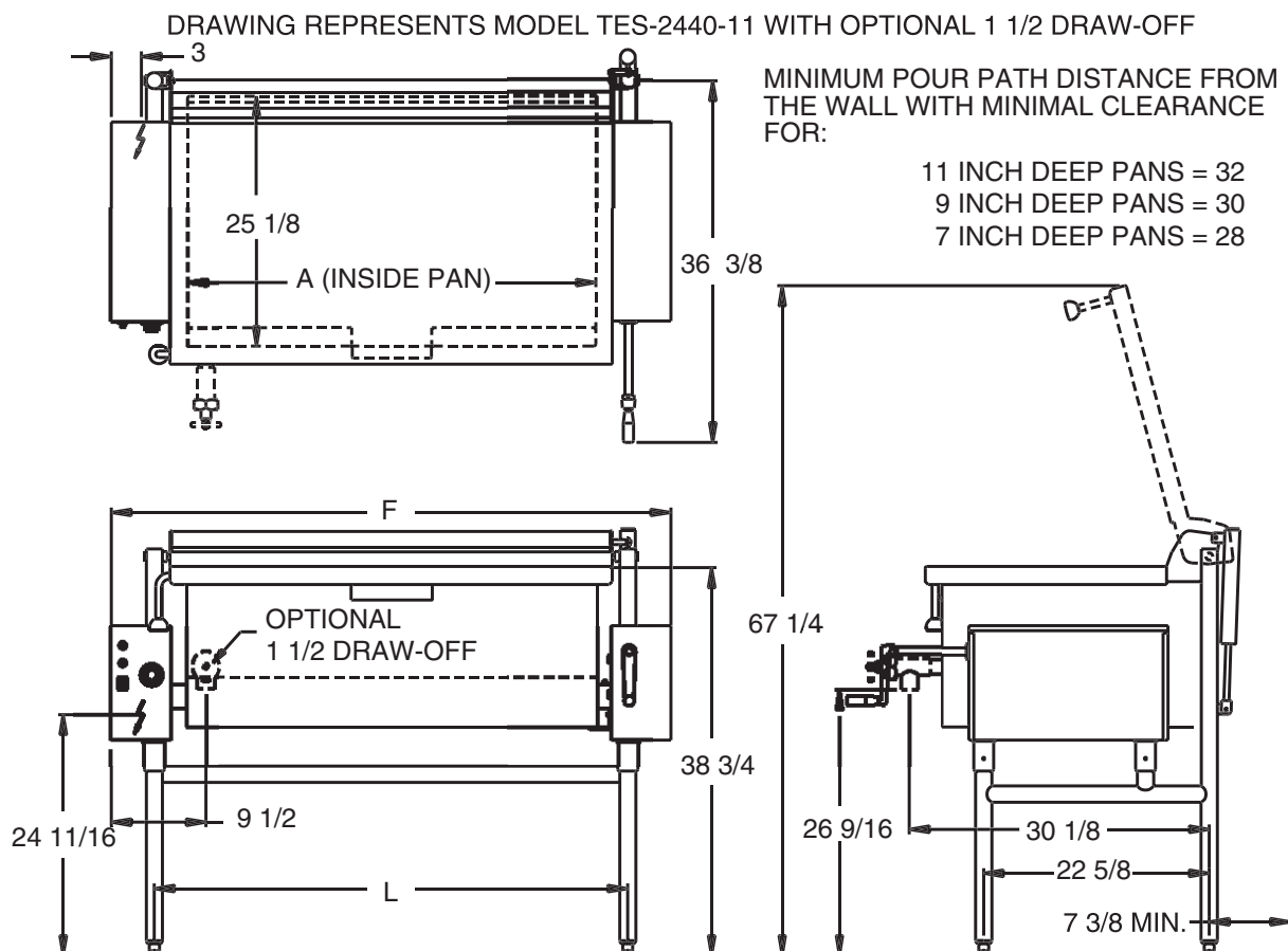
CLASSIC TILTING SKILLET MODEL TES DIMENSIONS
