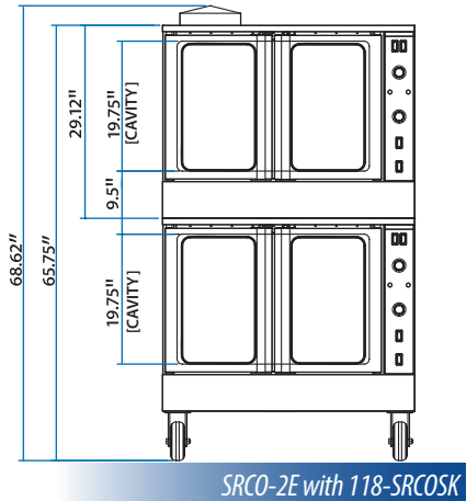
Dual Oven Configuration with Stacking Kit
