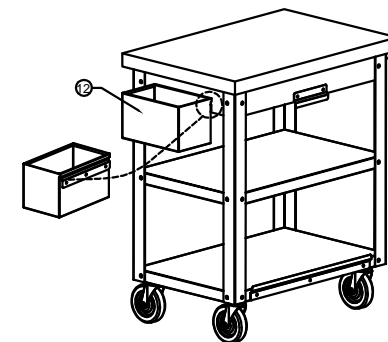
Final Assembly
