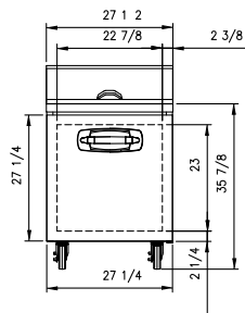
NLSMP27-12 ELEVATION VIEW
