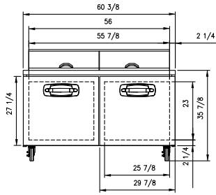
NLSMP60-24 ELEVATION VIEW
