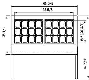
NLSMP60-24 PLAN VIEW
