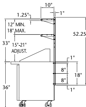
DOUBLE SHELF SIDE VIEW
