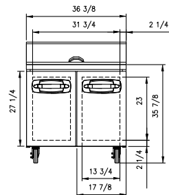
NLSMP36-15 ELEVATION VIEW
