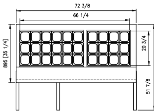
NLSMP72-30 PLAN VIEW
