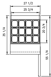
NLSMP27-12 PLAN VIEW
