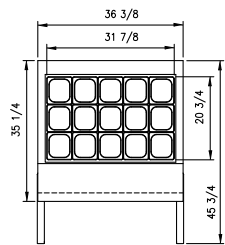
NLSMP36-15 PLAN VIEW
