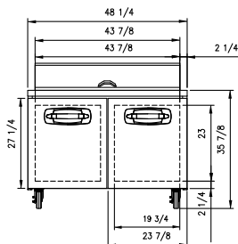
NLSMP48-18 ELEVATION VIEW
