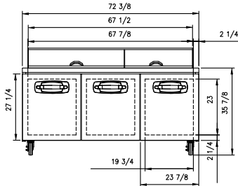
NLSMP72-30 ELEVATION VIEW
