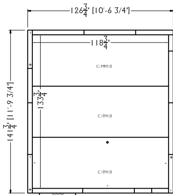
CEILING PANELS
