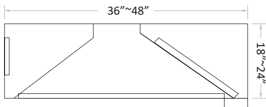
RMUA SERIES REGULAR EXHAUST WITH MAKE UP AIR W: 36" to 48" H: 18" to 24"
