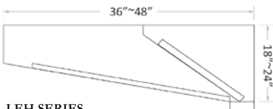
LEH SERIES LOW END EXHAUST HOODS W: 36" to 48" H: 18" to 24"
