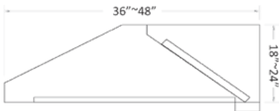
REH SERIES REGULAR EXHAUST HOODS W: 36" to 48" H: 18" to 24"
