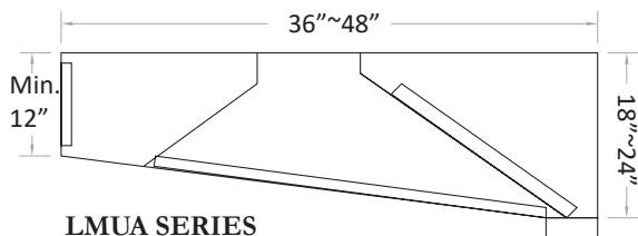
LMUA SERIES LOW END EXHAUST WITH MAKE UP AIR W: 36" to 48" H: 18" to 24"
