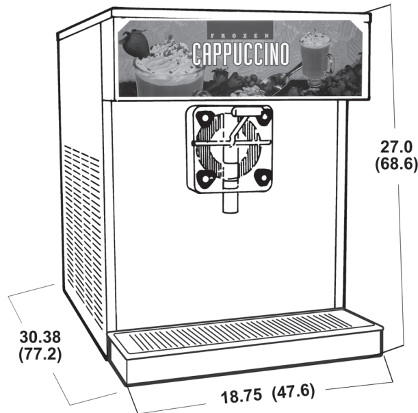
model 5711 represented measurements in inches [cm]
