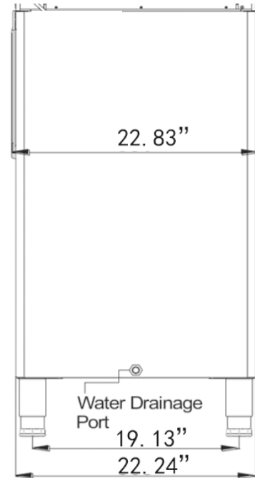
BACK VIEW
