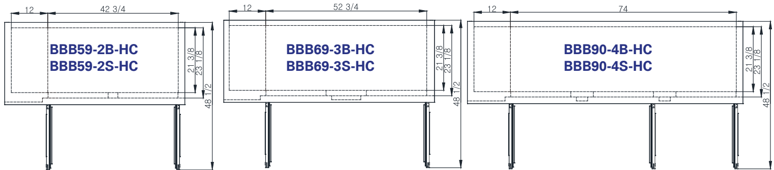
- Front View -
