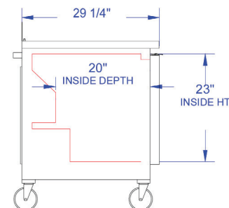
COMMON END
