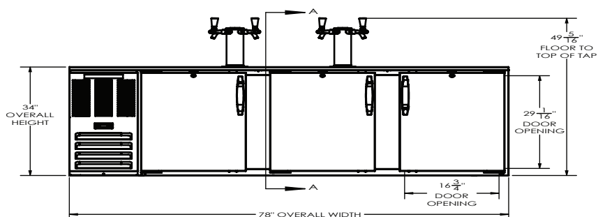
ELEVATION VIEW
