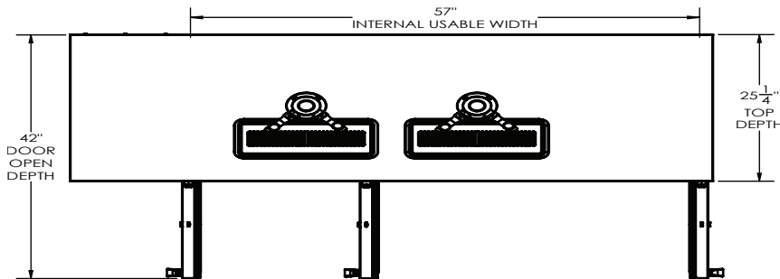
ELEVATION VIEW
