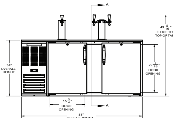
ELEVATION VIEW
