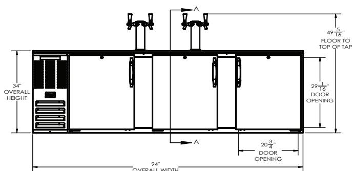
ELEVATION VIEW
