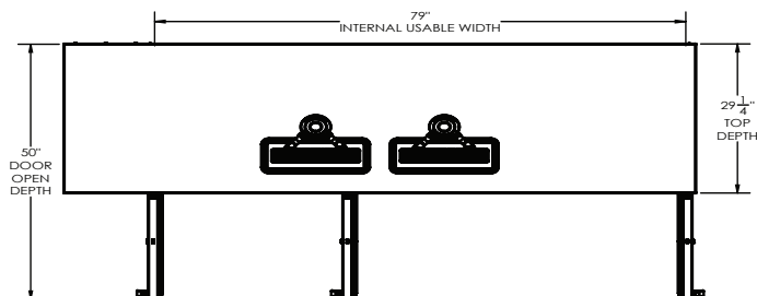
ELEVATION VIEW
