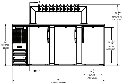
ELEVATION VIEW
