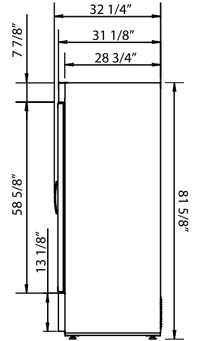
COMMON SIDE VIEW
