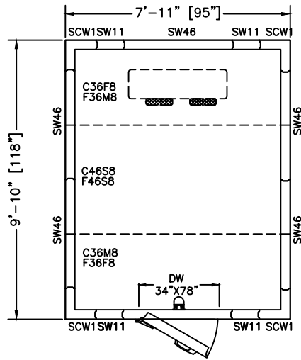
PLAN VIEW LEFT HINGE SELECT
