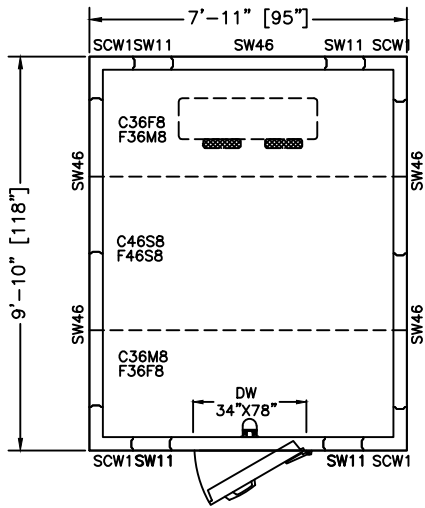
PLAN VIEW RIGHT HINGE SELECT
